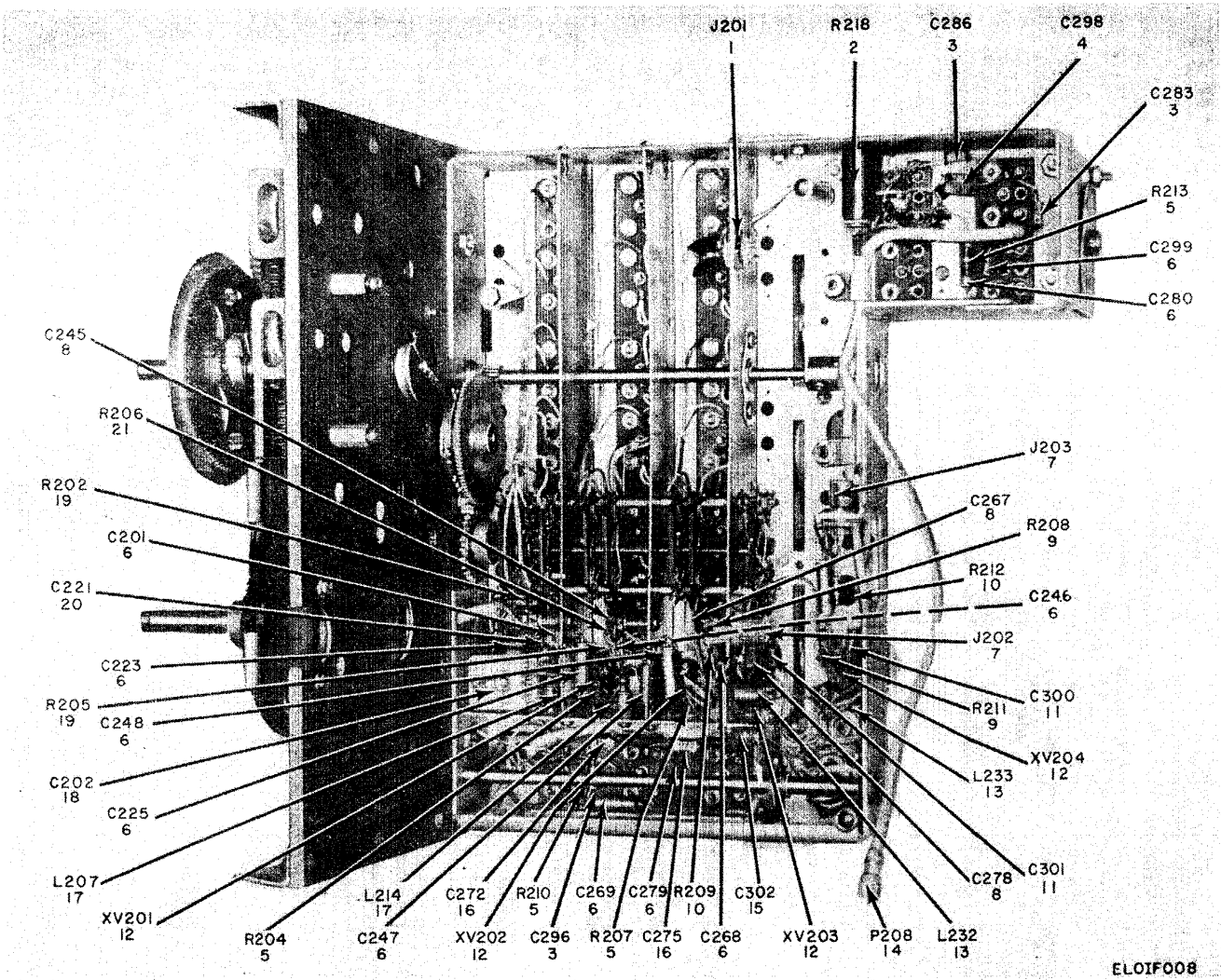
Figure 8. Amplifier, Radio Frequency, Full Bottom Interior View
