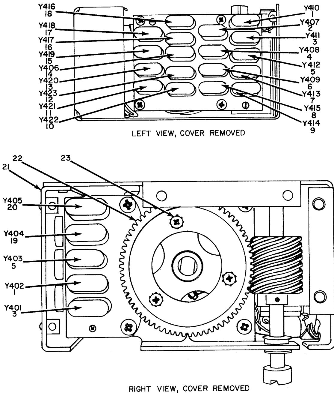
Figure 13. Oscillator, Radio Frequency, Crystal Controlled, Left and Right Views, Cover Removed.
